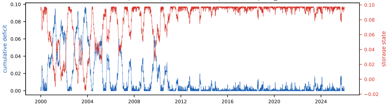
Real energy vs EIA demand (40 TWh/yr, 0.2% land)
