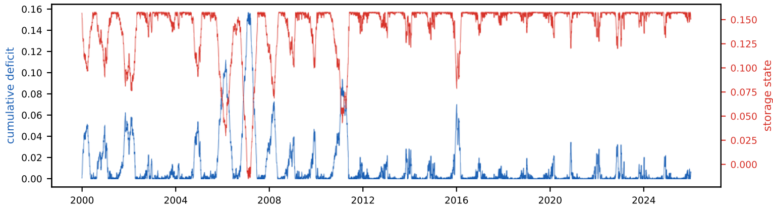
Cumulative deficit & storage state (peak deficit = required storage, S_{\text{tot}} =15.7% of annual)
