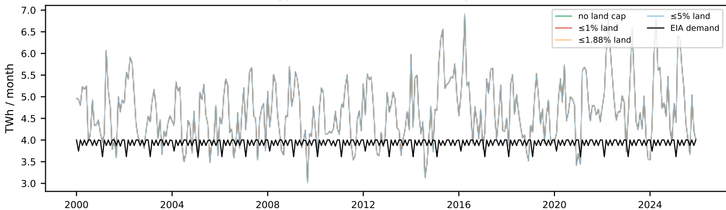
Real energy vs EIA demand (47 TWh/yr, 0.4% land)
