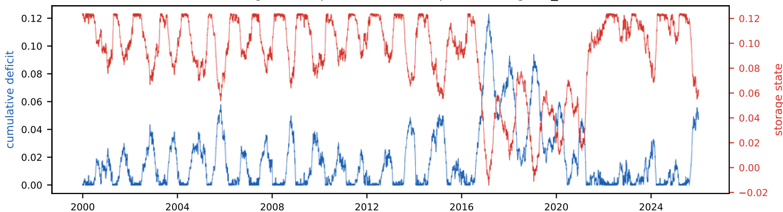
Real energy vs EIA demand (80 TWh/yr, 0.7% land)
