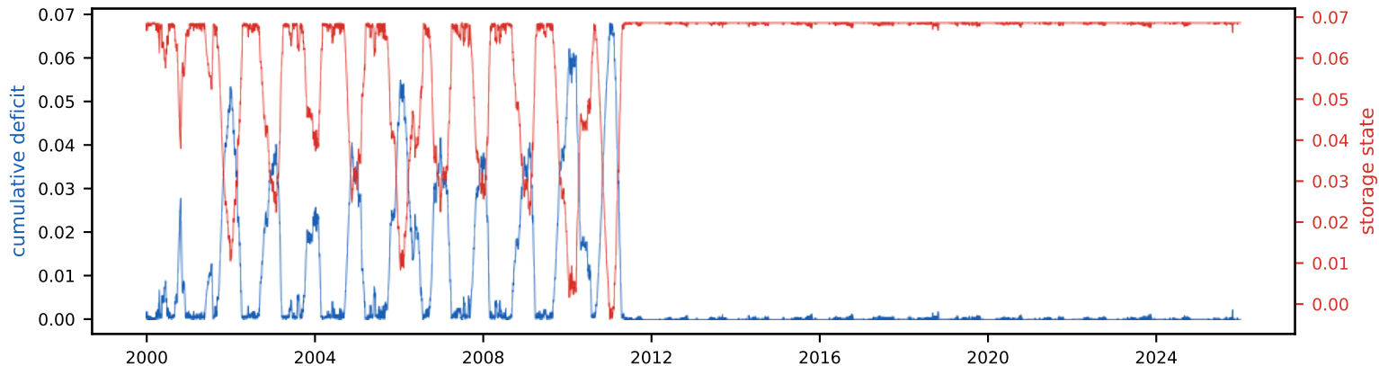
Cumulative deficit & storage state (peak deficit = required storage, S_{\text{tot}} =6.8% of annual)
