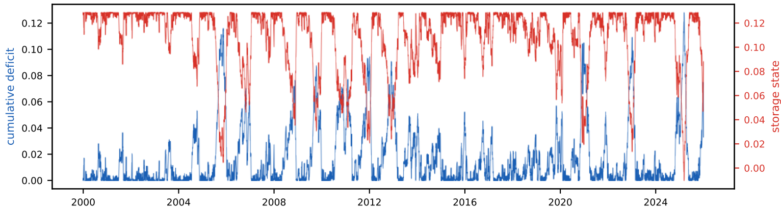
Cumulative deficit & storage state (peak deficit = required storage, S_{\text{tot}} =12.9% of annual)
