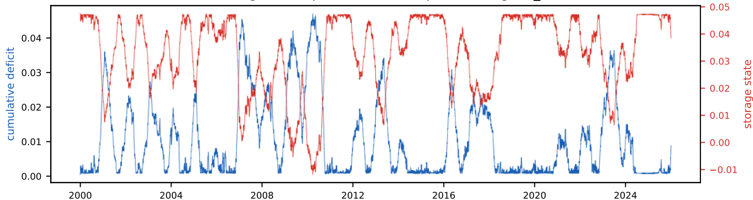
Cumulative deficit & storage state (peak deficit = required storage, S_{\text{tot}} =4.8% of annual)
