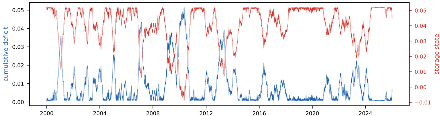
Cumulative deficit & storage state (peak deficit = required storage, S_{\text{tot}} =5.3% of annual)
