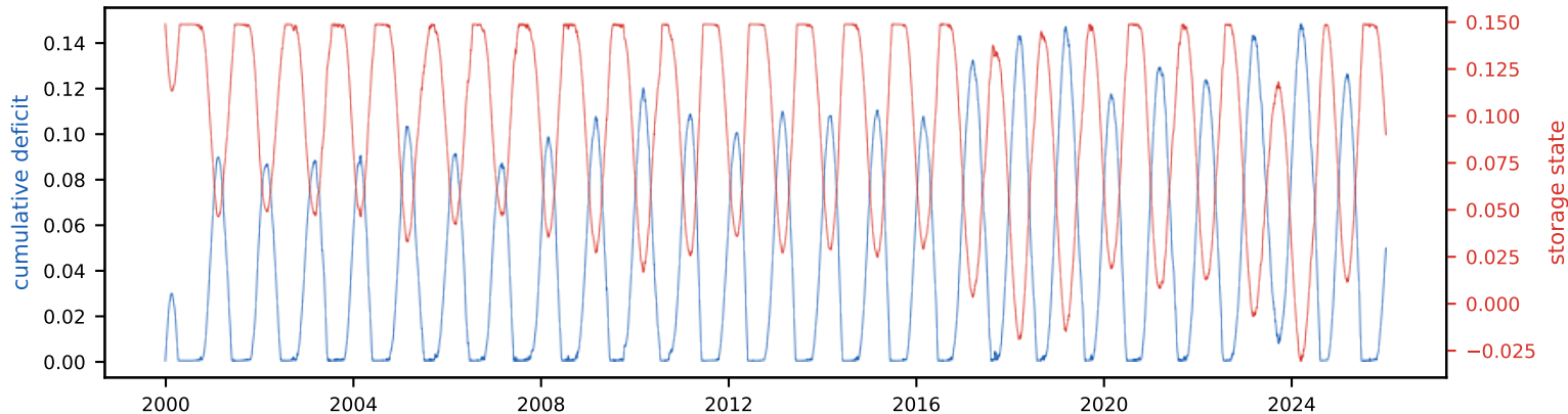
Cumulative deficit & storage state (peak deficit = required storage, S_{\text{tot}} =14.9% of annual)
