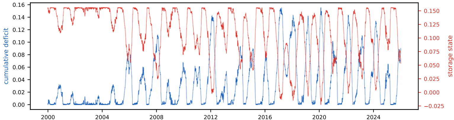
Cumulative deficit & storage state (peak deficit = required storage, S_{\text{tot}} =15.6% of annual)
