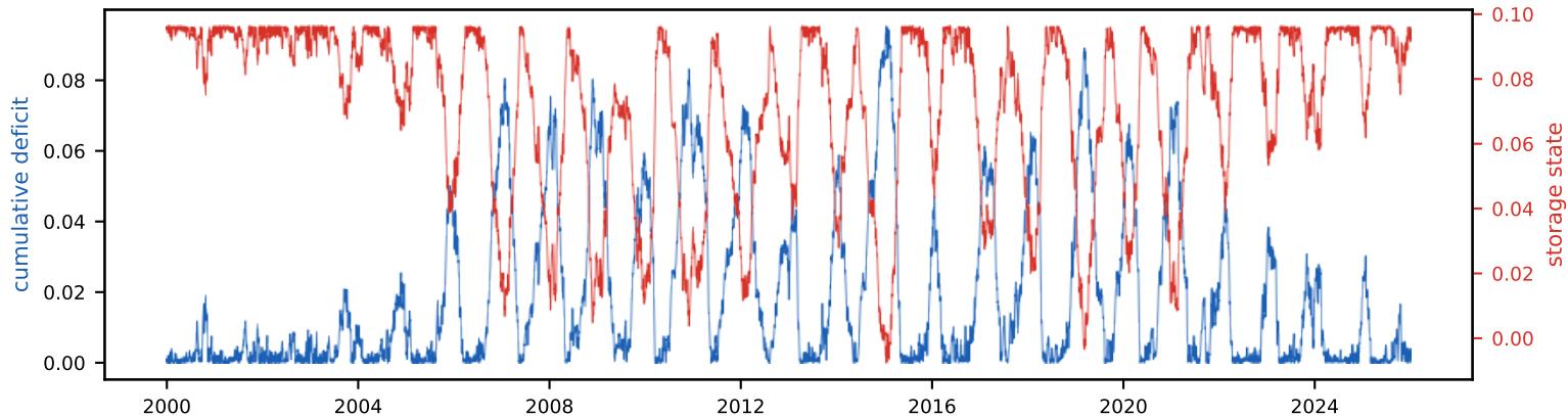
Cumulative deficit & storage state (peak deficit = required storage, S_{\text{tot}} =9.6% of annual)
