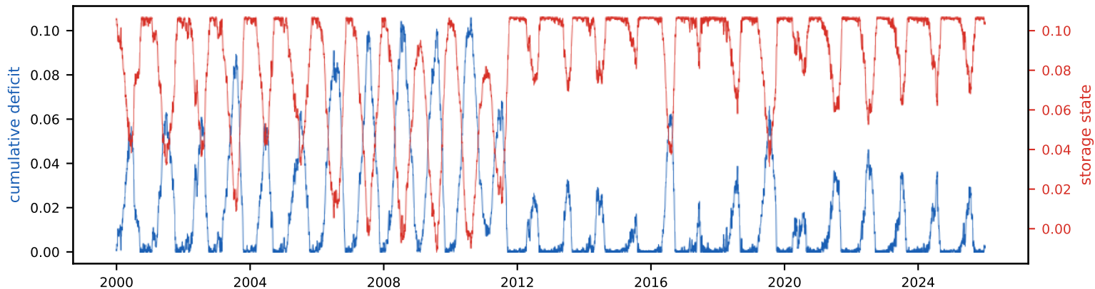
Cumulative deficit & storage state (peak deficit = required storage, S_{\text{tot}} =10.7% of annual)
