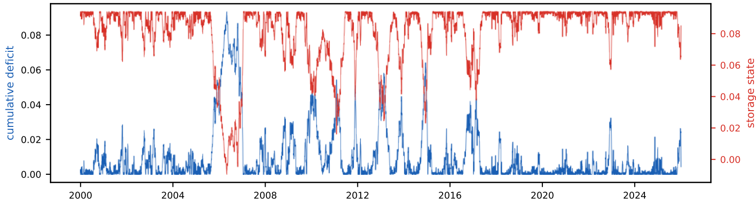
Cumulative deficit & storage state (peak deficit = required storage, S_{\text{tot}} =9.4% of annual)
