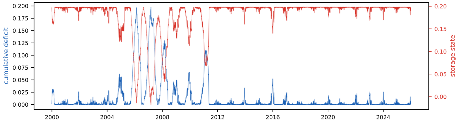
Cumulative deficit & storage state (peak deficit = required storage, S_{tot} =19.8% of annual)
