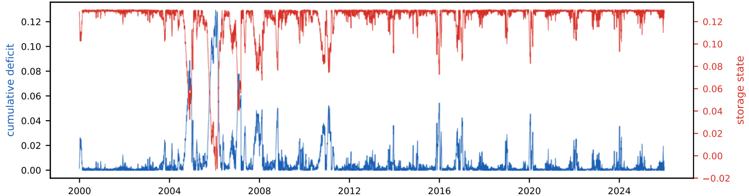
Cumulative deficit & storage state (peak deficit = required storage, S_{\text{tot}} =13.0% of annual)
