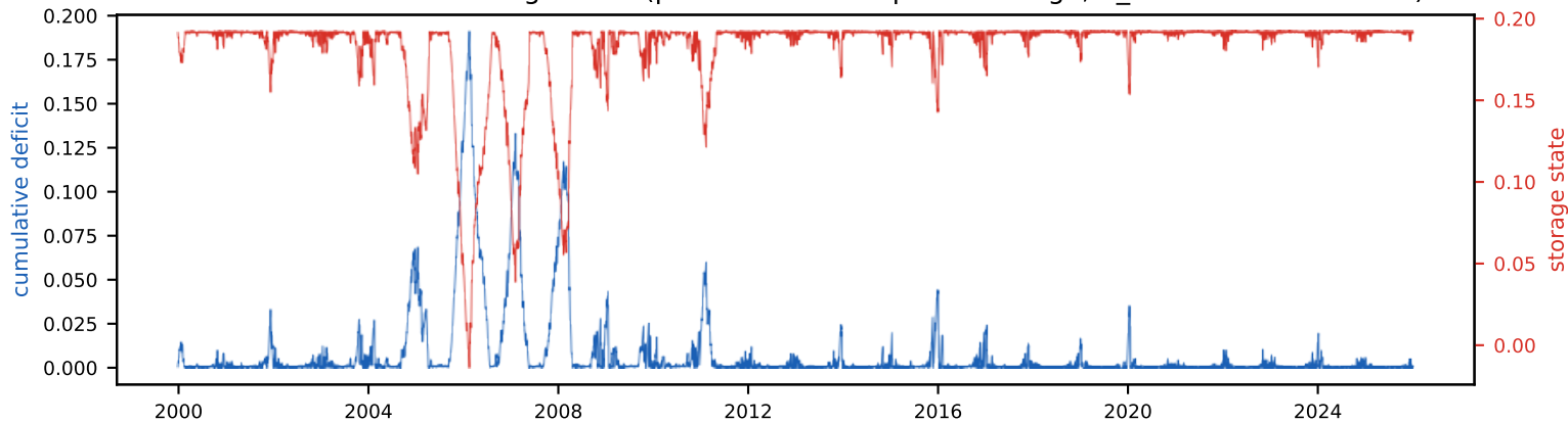
Cumulative deficit & storage state (peak deficit = required storage, S_{\text{tot}} =19.2% of annual)
