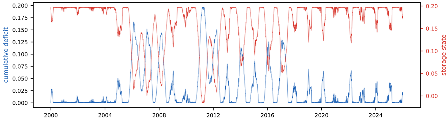
Cumulative deficit & storage state (peak deficit = required storage, S_{tot} =19.7% of annual)
