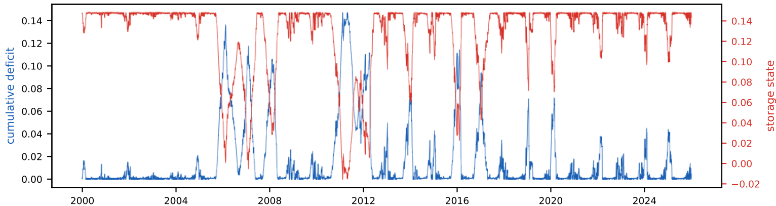
Cumulative deficit & storage state (peak deficit = required storage, S_{\text{tot}} =14.8% of annual)
