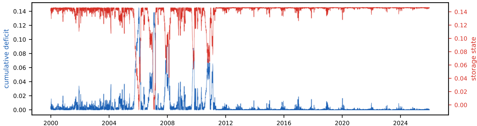
Cumulative deficit & storage state (peak deficit = required storage, S_{\text{tot}} =14.6% of annual)
