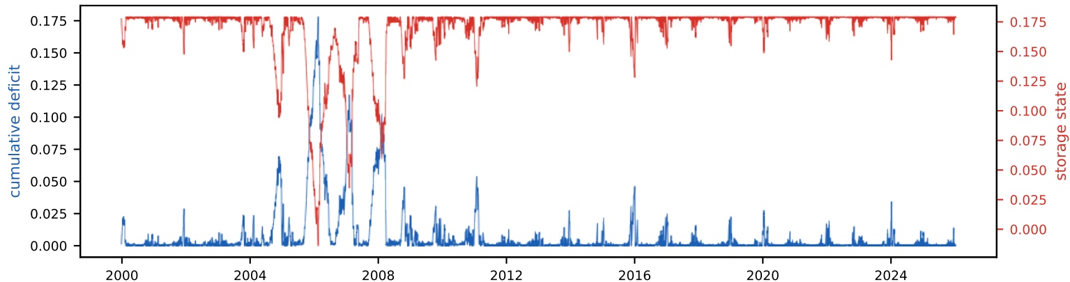
Cumulative deficit & storage state (peak deficit = required storage, S_{\text{tot}} =17.9% of annual)
