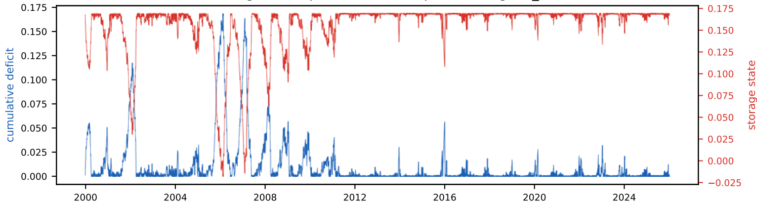
Cumulative deficit & storage state (peak deficit = required storage, S_{\text{tot}} =16.9% of annual)
