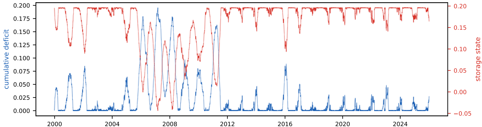
Cumulative deficit & storage state (peak deficit = required storage, S_{\text{tot}} =19.6% of annual)
