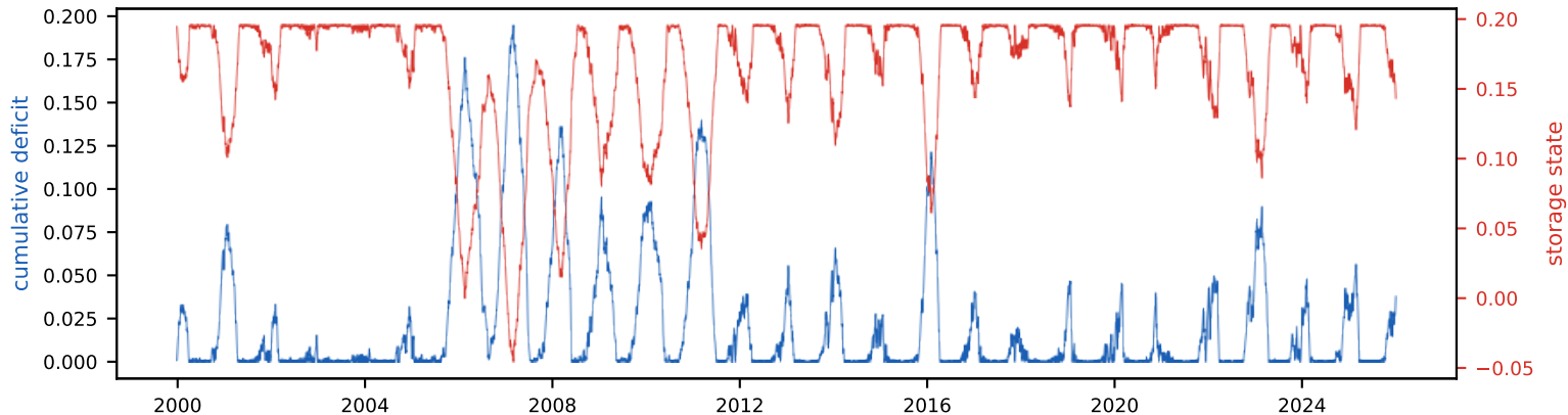
Cumulative deficit & storage state (peak deficit = required storage, S_{\text{tot}} =19.5% of annual)
