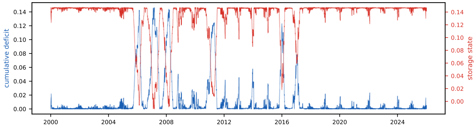
Cumulative deficit & storage state (peak deficit = required storage, S_{\text{tot}} =14.7% of annual)
