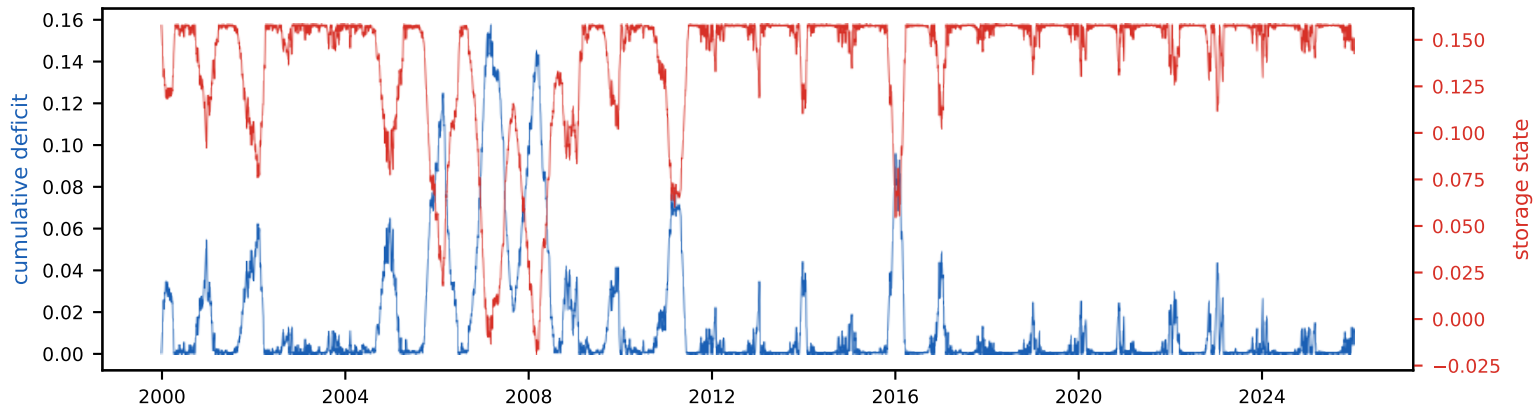
Cumulative deficit & storage state (peak deficit = required storage, S_{\text{tot}} =15.8% of annual)
