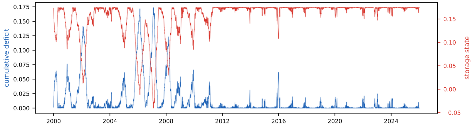
Cumulative deficit & storage state (peak deficit = required storage, S_{\text{tot}} =17.4% of annual)
