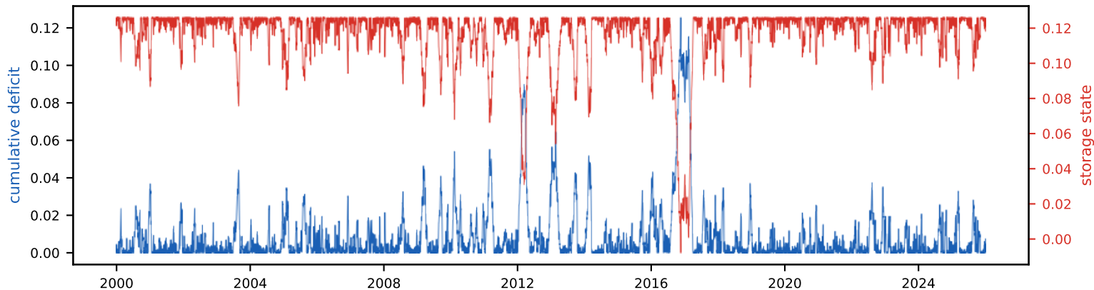
Cumulative deficit & storage state (peak deficit = required storage, S_{\text{tot}}=12.6\% of annual)
