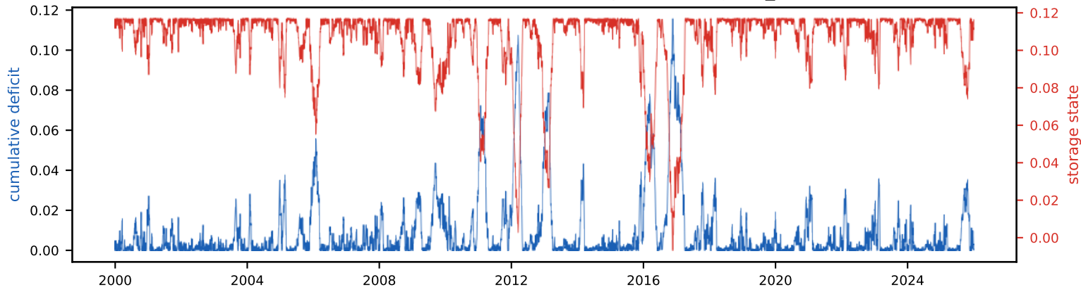
Cumulative deficit & storage state (peak deficit = required storage, S_{\text{tot}} =11.7% of annual)
