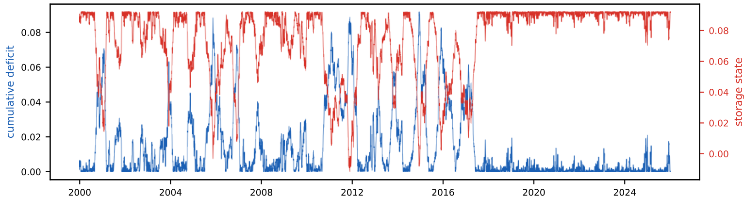
Cumulative deficit & storage state (peak deficit = required storage, S_{tot}=9.2\% of annual)
