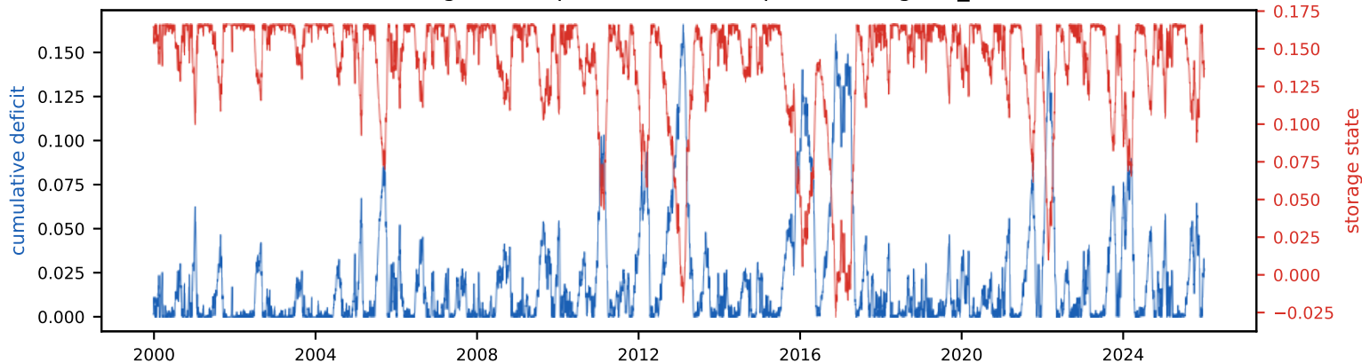
Cumulative deficit & storage state (peak deficit = required storage, S_{\text{tot}} =16.6% of annual)
