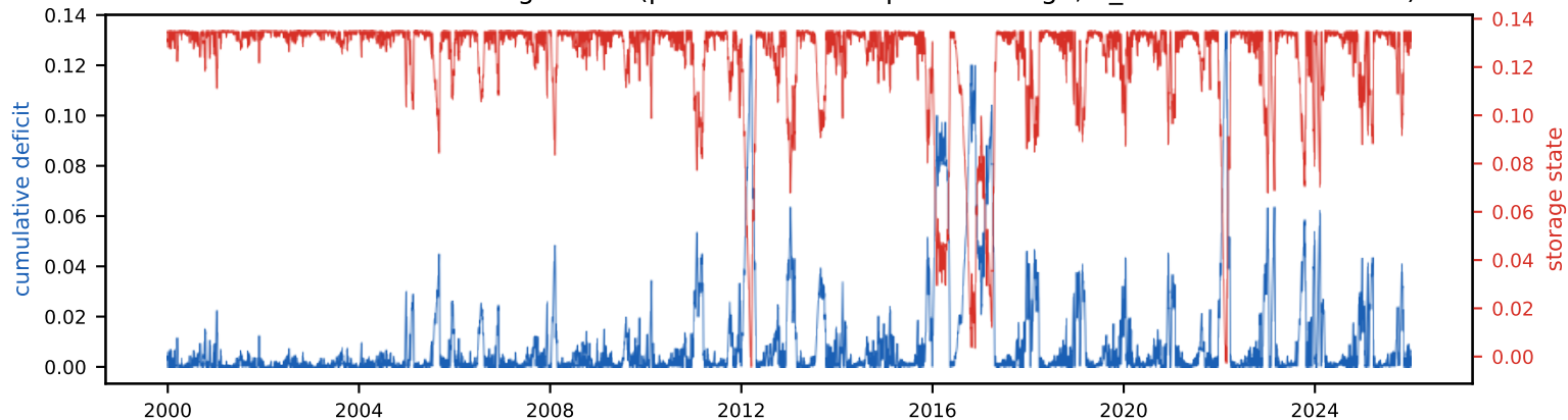
Cumulative deficit & storage state (peak deficit = required storage, S_{\text{tot}} =13.5% of annual)
