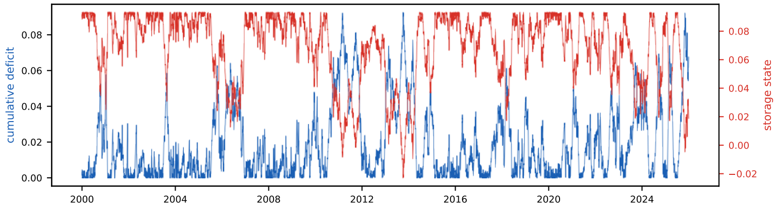
Cumulative deficit & storage state (peak deficit = required storage, S_{\text{tot}} =9.3% of annual)
