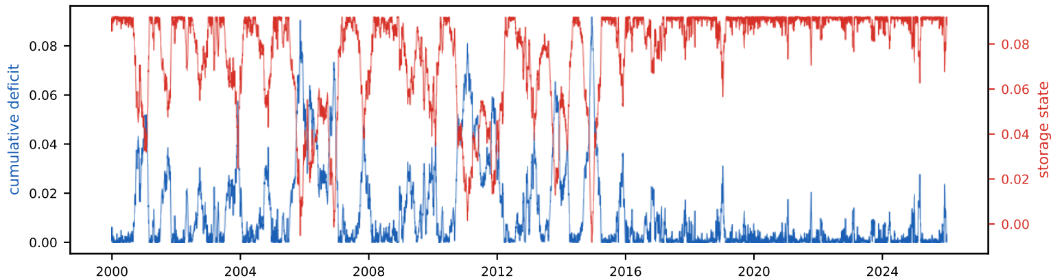
Cumulative deficit & storage state (peak deficit = required storage, S_{\text{tot}} =9.2% of annual)
