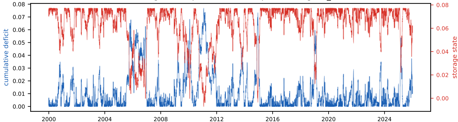
Cumulative deficit & storage state (peak deficit = required storage, S_{\text{tot}}=7.7\% of annual)
