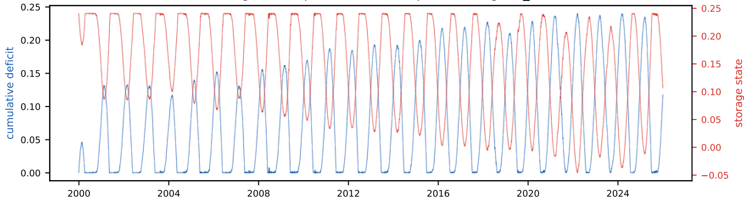
Cumulative deficit & storage state (peak deficit = required storage, S_{\text{tot}} =24.1% of annual)
