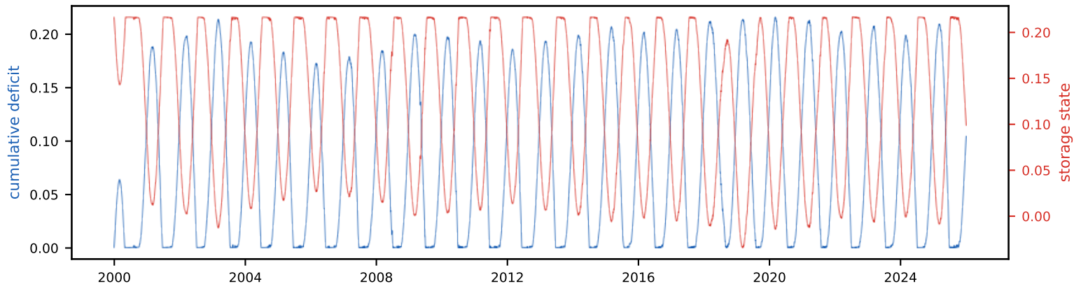
Cumulative deficit & storage state (peak deficit = required storage, S_{\text{tot}} =21.7% of annual)
