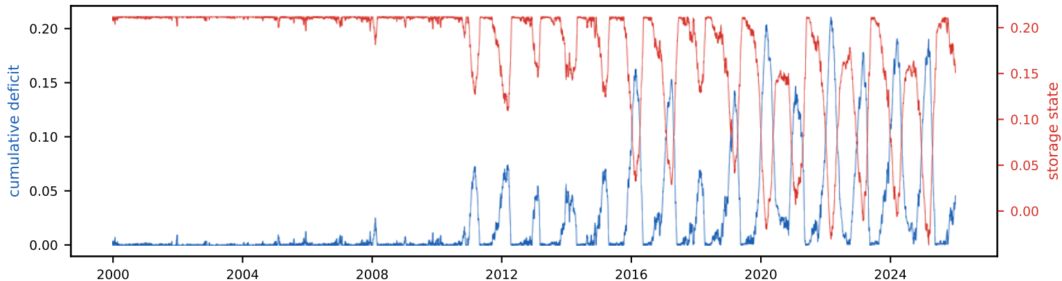
Cumulative deficit & storage state (peak deficit = required storage, S_{\text{tot}} =21.1% of annual)
