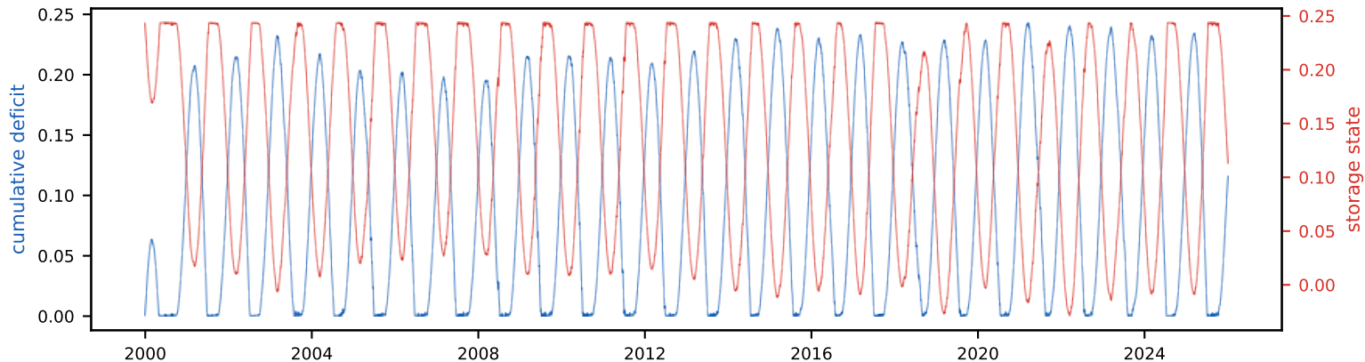
Cumulative deficit & storage state (peak deficit = required storage, S_{\text{tot}} =24.4% of annual)
