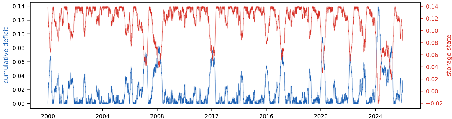
Cumulative deficit & storage state (peak deficit = required storage, S_{\text{tot}} =13.9% of annual)
