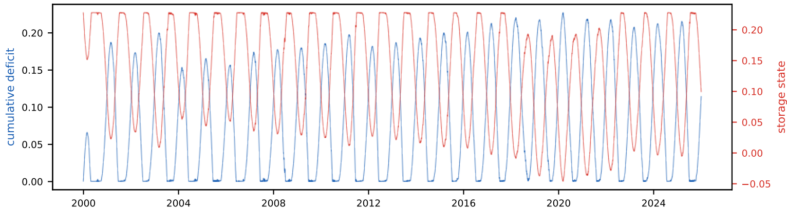
Cumulative deficit & storage state (peak deficit = required storage, S_{\text{tot}} =22.8% of annual)
