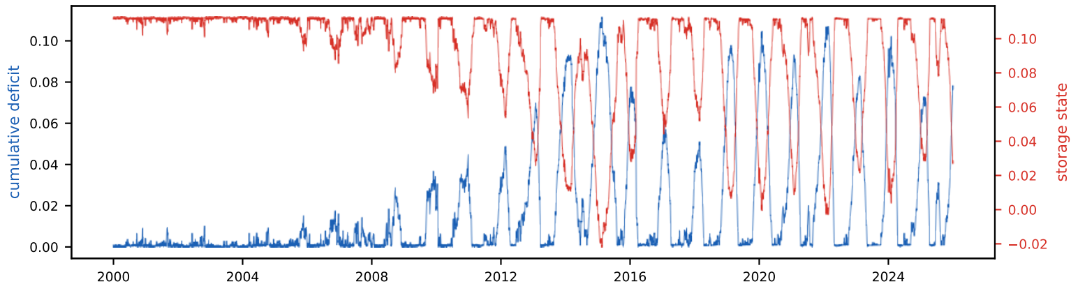
Cumulative deficit & storage state (peak deficit = required storage, S_{\text{tot}} =11.2% of annual)
