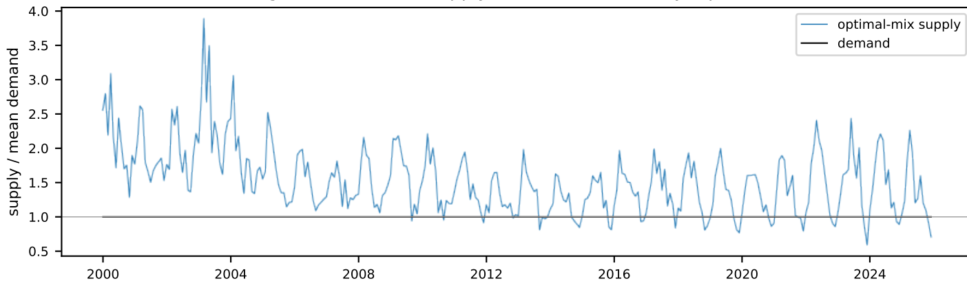
Hidalgo — normalized supply vs demand (monthly, optimal mix)
