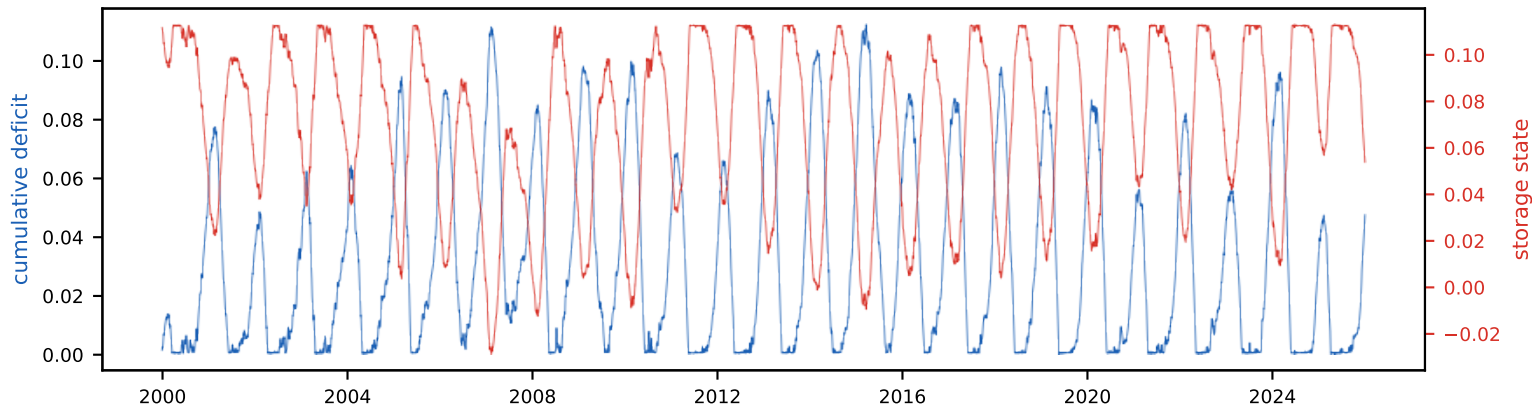
Cumulative deficit & storage state (peak deficit = required storage, S_{\text{tot}} =11.3% of annual)
