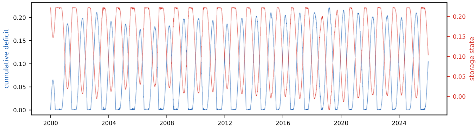
Cumulative deficit & storage state (peak deficit = required storage, S_{\text{tot}} =22.2% of annual)
