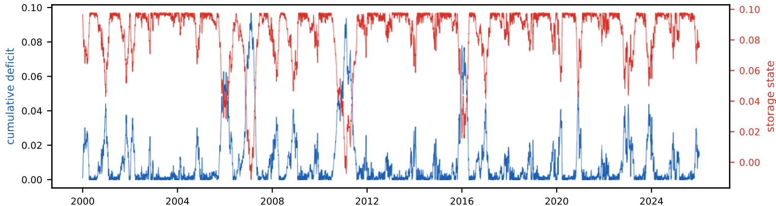
Cumulative deficit & storage state (peak deficit = required storage, S_{\text{tot}} =9.8% of annual)
