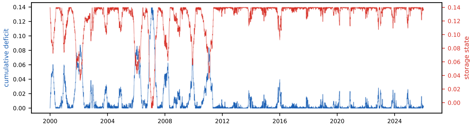
Cumulative deficit & storage state (peak deficit = required storage, S_{\text{tot}} =14.0% of annual)
