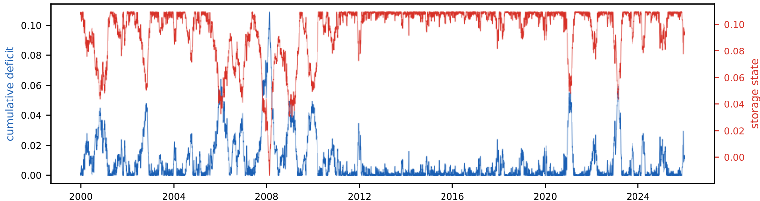
Cumulative deficit & storage state (peak deficit = required storage, S_{\text{tot}} =10.9% of annual)
