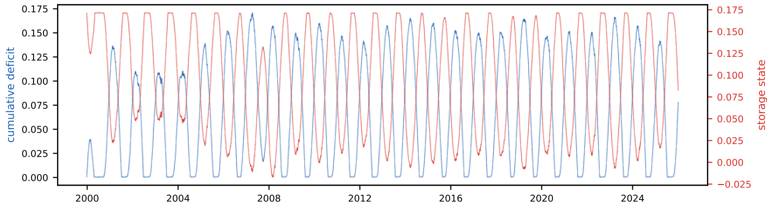
Cumulative deficit & storage state (peak deficit = required storage, S_{\text{tot}} =17.2% of annual)
