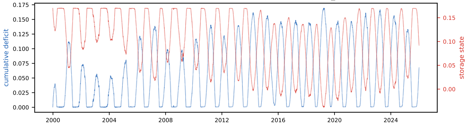
Cumulative deficit & storage state (peak deficit = required storage, S_{\text{tot}} =17.0% of annual)
