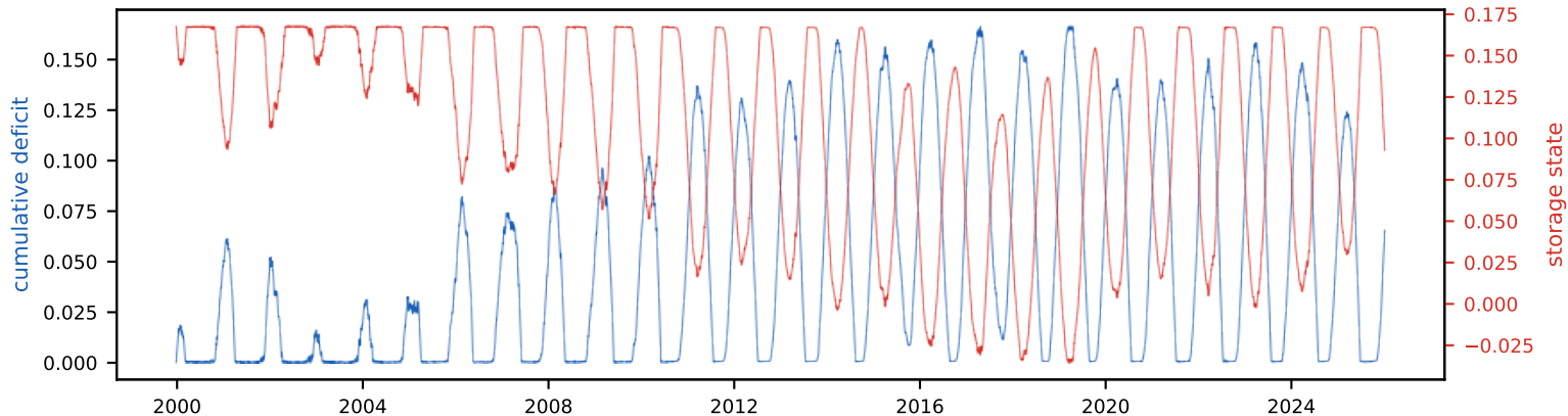
Cumulative deficit & storage state (peak deficit = required storage, S_{\text{tot}} =16.8% of annual)
