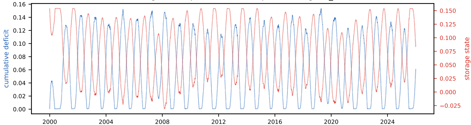
Cumulative deficit & storage state (peak deficit = required storage, S_{\text{tot}} =15.5% of annual)
